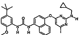
1-(5-tert-Butyl-2-methoxy-phenyl)-3-{4-[2-(cyclopropylmethyl-amino)-6-methyl-pyrimidin-4-yloxy]-naphthalen-1-yl}-urea;
